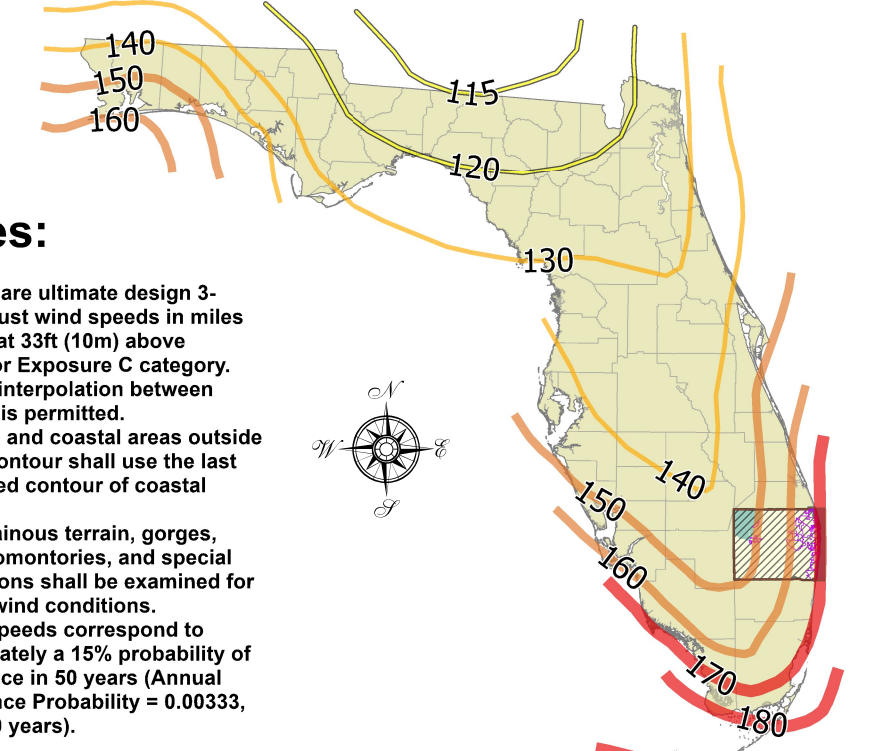
Figure 1609.3(1) Ultimate Design Wind Speeds, for Risk Category II Buildings and Other Structures
