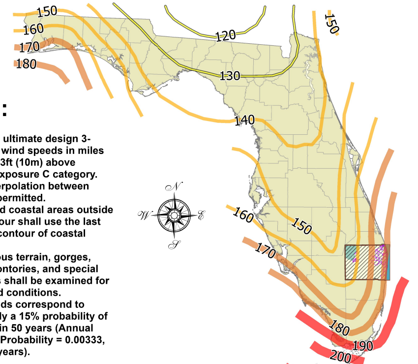
Figure 1609.3(2) Ultimate Design Wind Speeds, for Risk Category III Buildings and Other Structures
