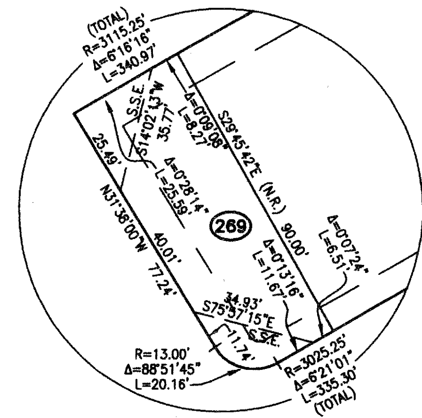
DETAIL "H" (NOT-TO-SCALE)
