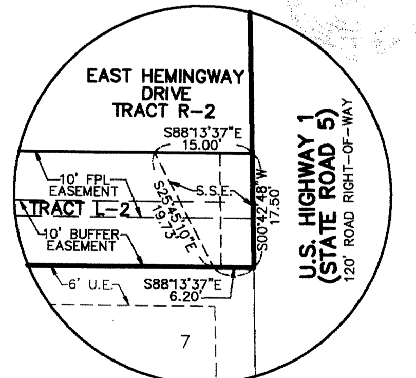
SAFE SITE EASEMENT DETAIL D NOT TO SCALE
