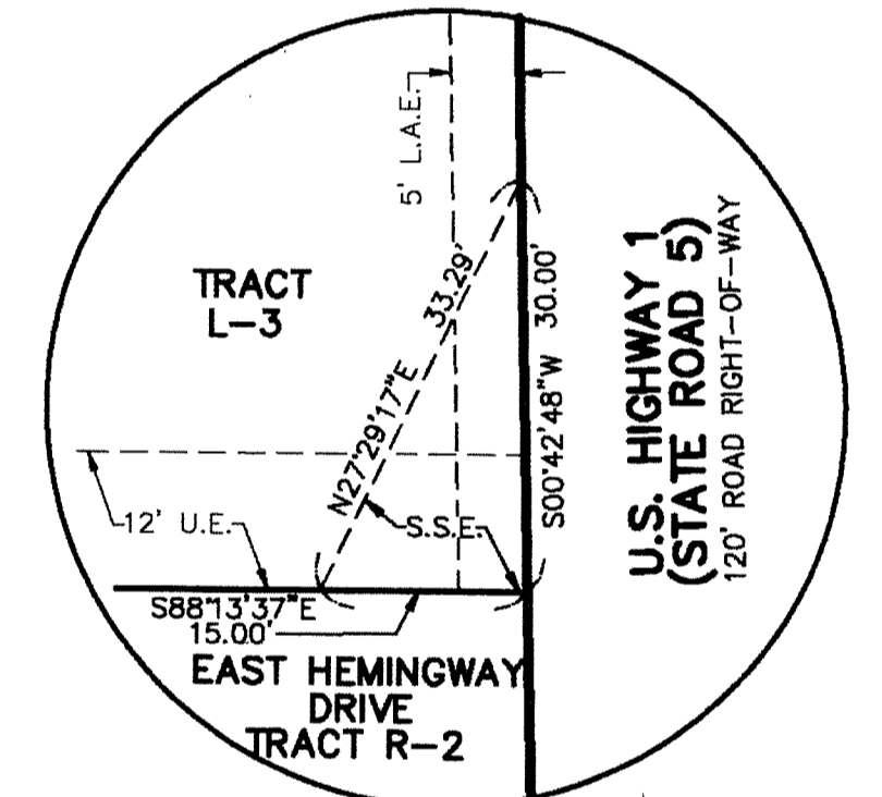
SAFE SITE EASEMENT DETAIL C NOT TO SCALE
