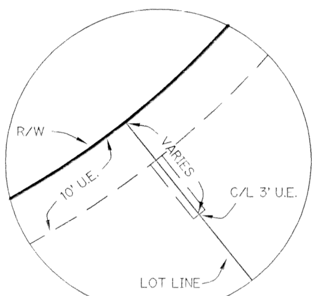
DETAIL "A" (TYPICAL 3' UTILITY EASEMENT) N.T.S.
