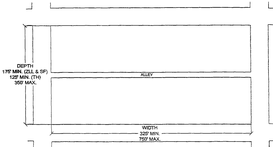
Figure 3.2 – Residential Block Structure
