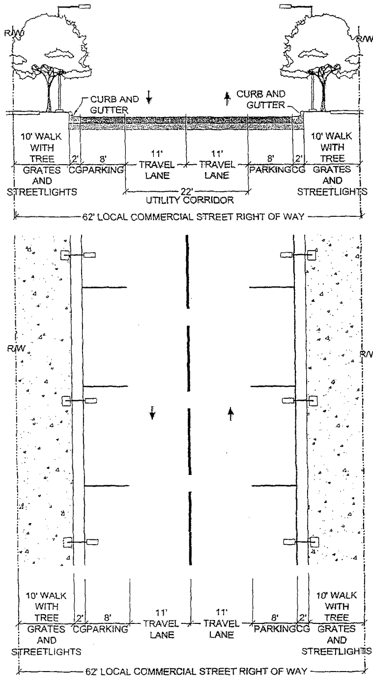
Figure 5.5 –Local Commercial Street (Tertiary) 62' Right-of-Way Cross-Section
