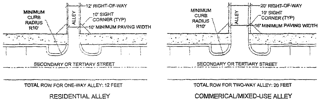
Figure 5.7 –Alley Design Standards
