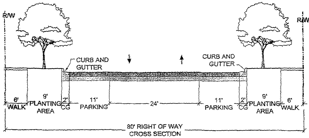
Figure 5.4 –Secondary Street 80' Right-of-Way Cross-Section with On-Street Parking
