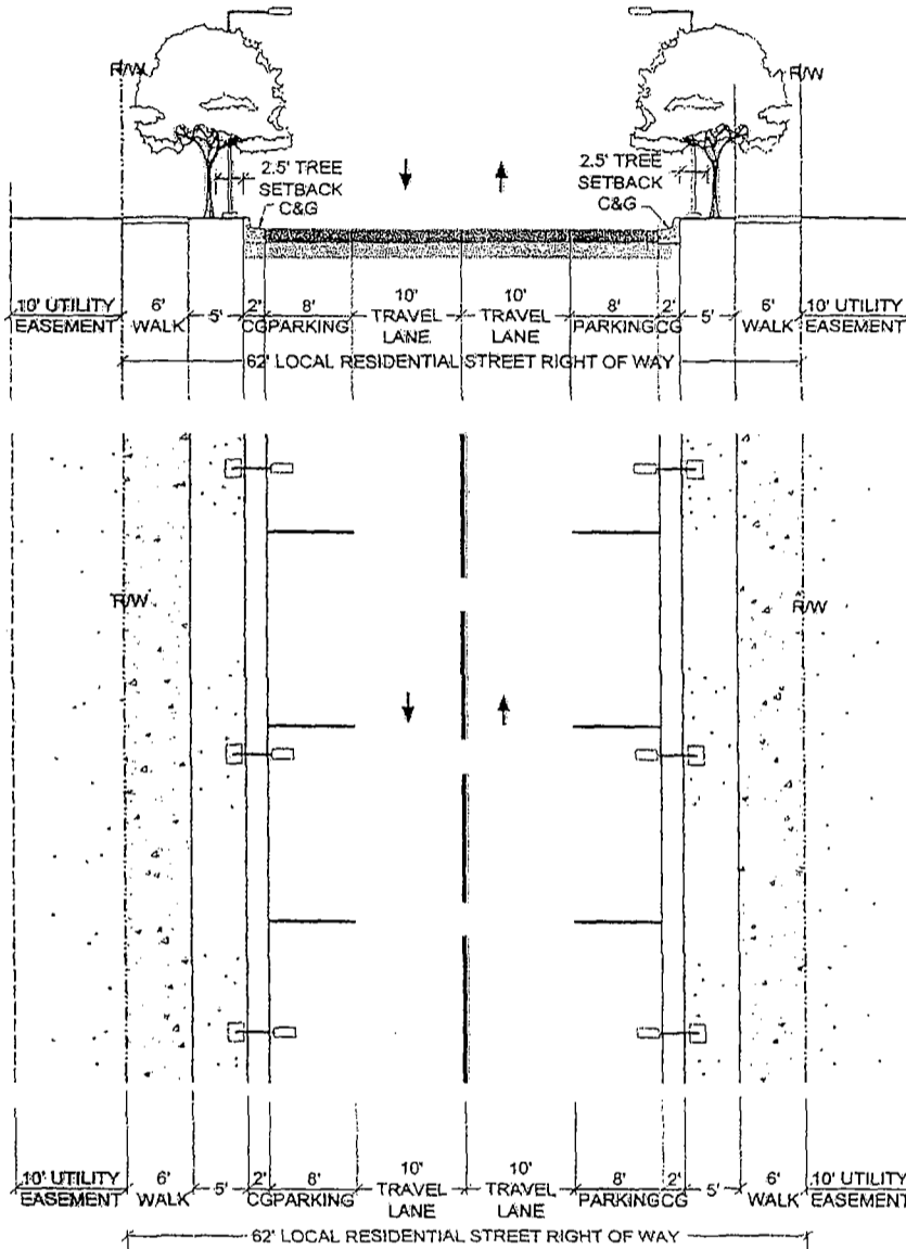
Figure 5.6 –Local Residential Street 62' Right-of-Way Cross-Section
