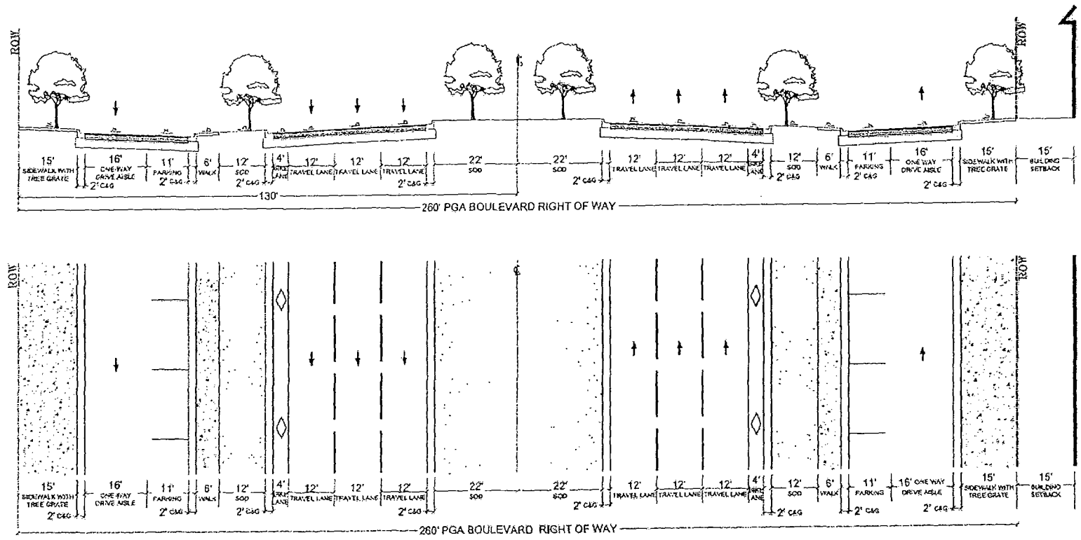
Figure 5.1 – PGA Boulevard 260' Right-of-Way Cross-Section
