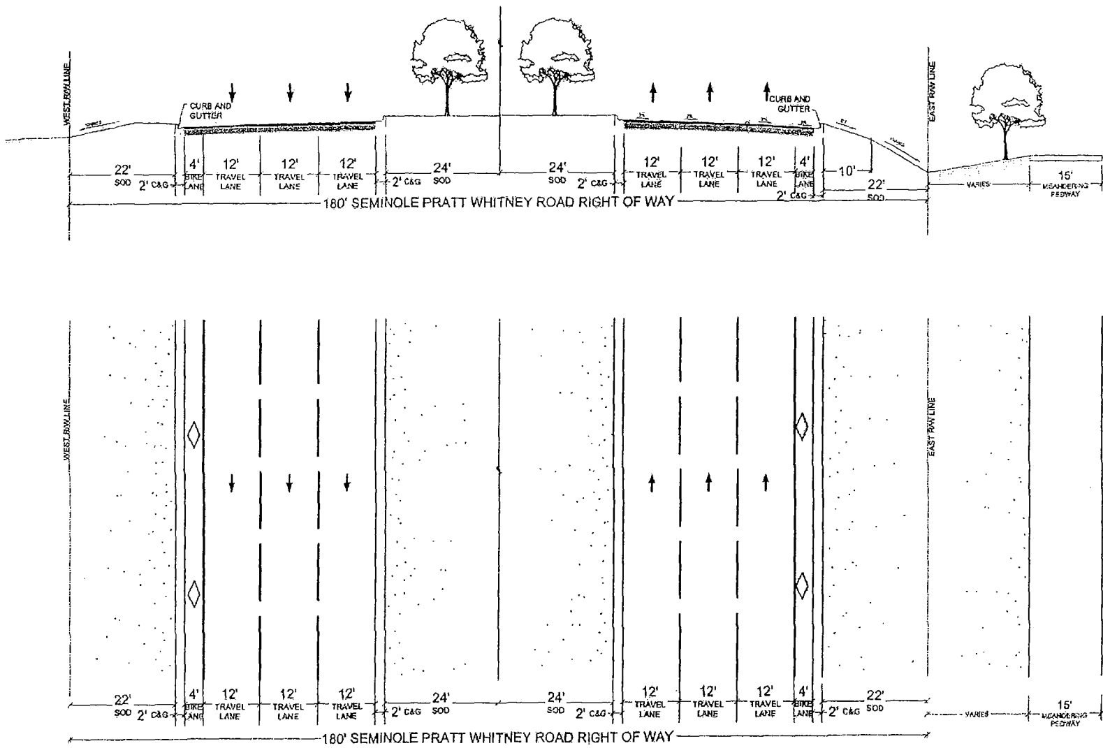
Figure 5.2 - Seminole Pratt Whitney Road 180' Right-of-Way Cross-Section
