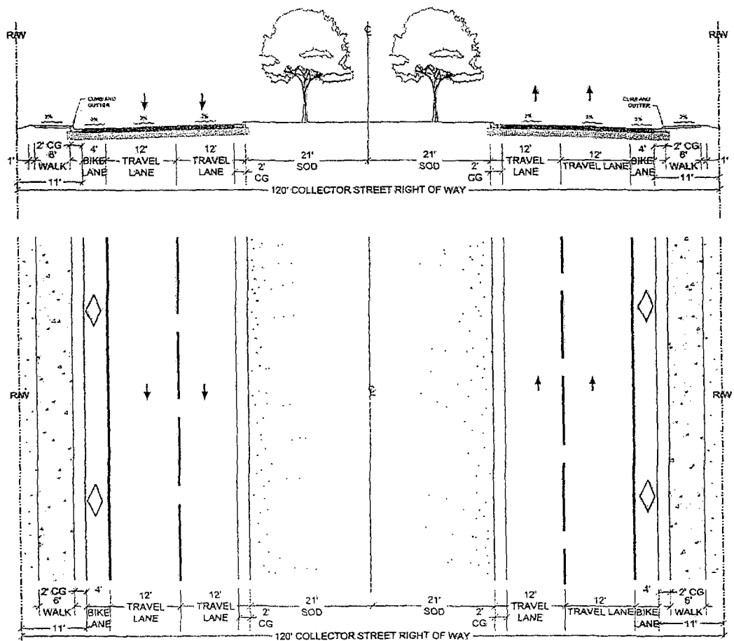
Figure 5.3 – Secondary (Collector) Street 120' Right-of-Way Cross-Section
